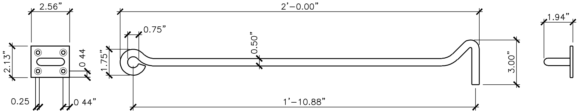
FRONT
